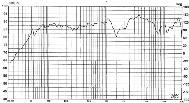
SPL vs Frequency, -35 Sweep
