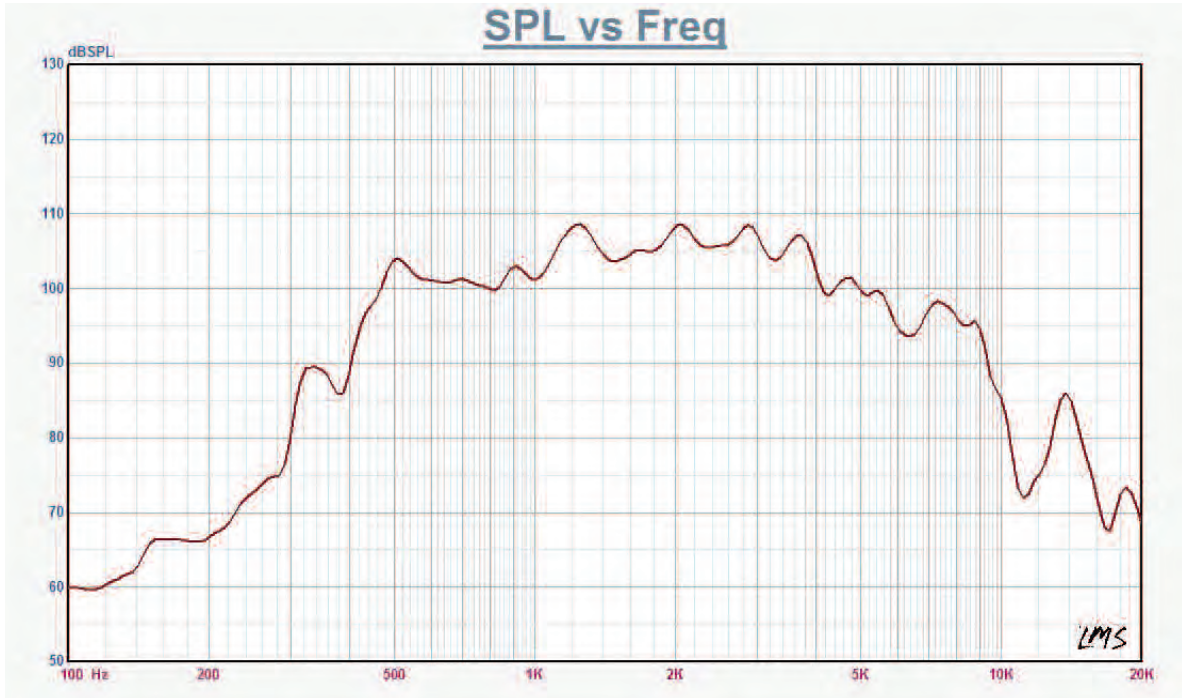
Measured with 1W input on rated impedance at 1m distance on speaker front axis and without transformer
